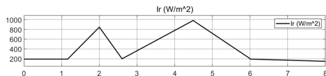
FIGURE 7. Irradiation pattern of PVs.
