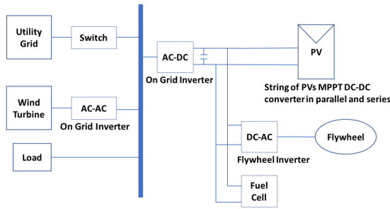
FIGURE 1. System Topology.
