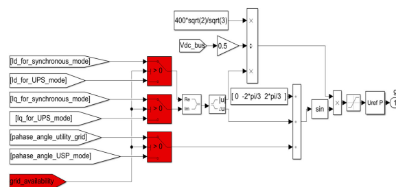
FIGURE 5. Control diagram of the inverter.
