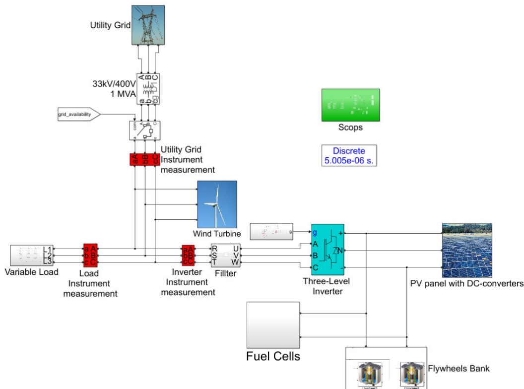
FIGURE 2. A Simulink screenshot of the MG.
