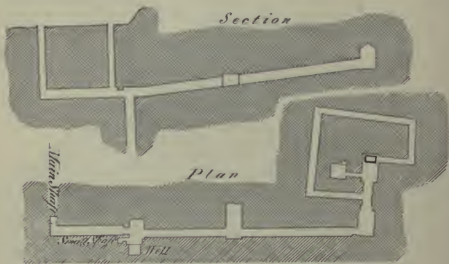
FIG. 101.—Section and plan of passages in pyramid of Illahun. Scale 1/1000.
