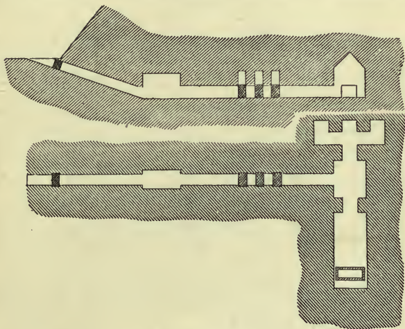
FIG. 50.—Section and plan of passages of the pyramid of Unas. Scale \frac{1}{8}\frac{1}{10} .
