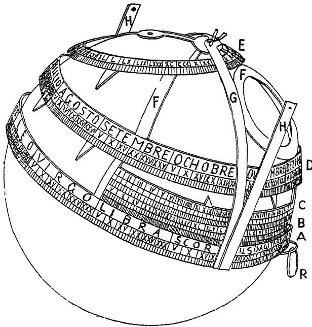
FIG 37. Spherical astrolabe of Alfonso the Wise of Castille, constructed for him by his Jewish astronomers and described and figured by them. It is here exhibited as reconstructed. The sphere itself is not an essential part of the instrument, which is complete provided all the circles and bands are present. A is a circle marked with the twelve signs of the zodiac, each of which is graduated into thirty divisions. B C is a band of variously graduated quadrants. D is a calendarium bearing the Castilian names of the months, each of which is graduated into the appropriate number of days. E is the equator. F is a connecting piece used to give mechanical strength. G is the so-called Alidad , that is to say the movable part of the astrolabe that carries a sight . The Alidad rotates around an axis and the amount of rotation can be read off against the quadrants and circles. The sights themselves are seen as small holes in the projecting pieces H H. One of these pieces is attached to the Alidad G. R is the ring from which the astrolabe is suspended.
