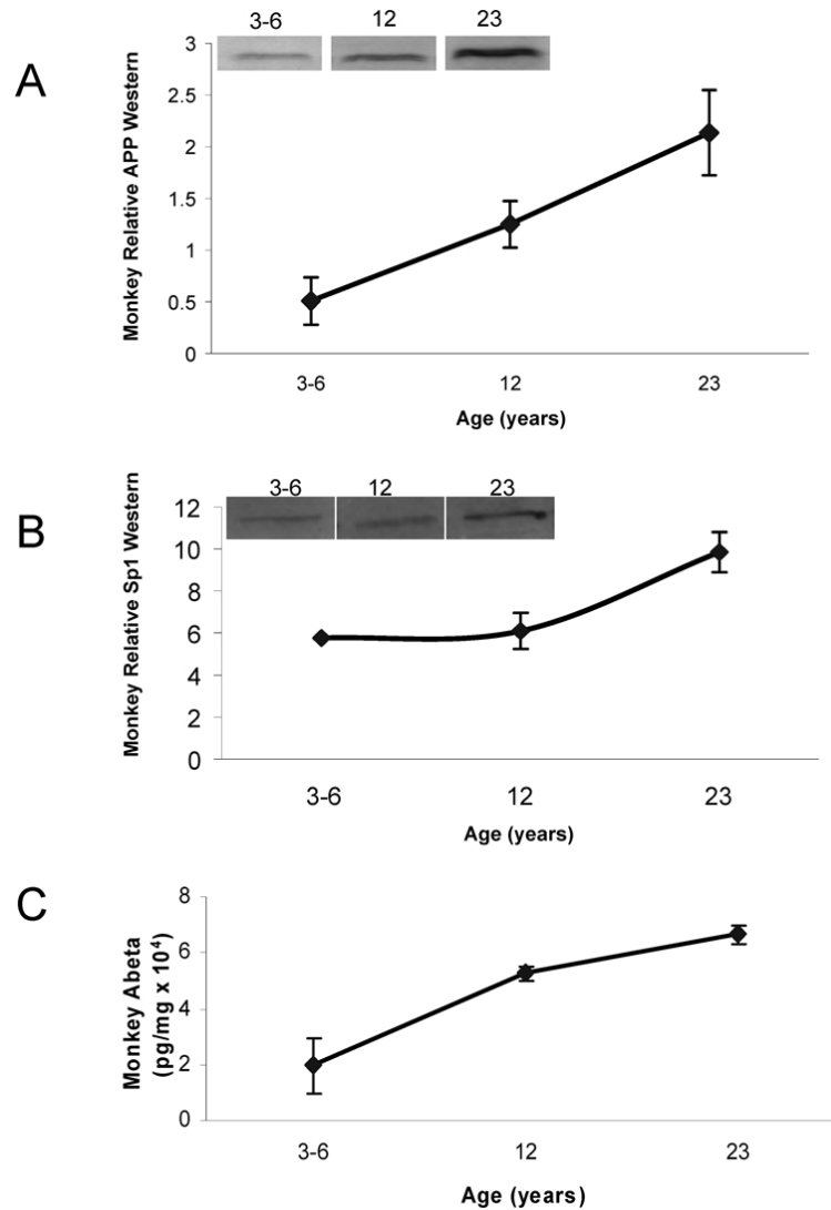
Fig. 4. Lifespan profile of AD related proteins ( A\beta PP, SP1, and A\beta ) in the primate brain. Protein from cortical tissue of Cynomolgus primate was isolated and probed with 22C11 A\beta PP N-terminus antibody with SDS-PAGE western blot analysis as described in the text. The SP1 antibody used is mentioned in the methods section. Protein was also used to measure A\beta_{1-40} using an ELISA assay (IBL, Japan). A) Relative A\beta PP protein signal; B) Relative SP1 signal; C. A\beta_{40} levels. Each data point in the curve is the mean + SEM ( n = 3 monkeys). Western blot results were normalized to \beta -actin signal. Representative blots are shown in insets for western analysis.
