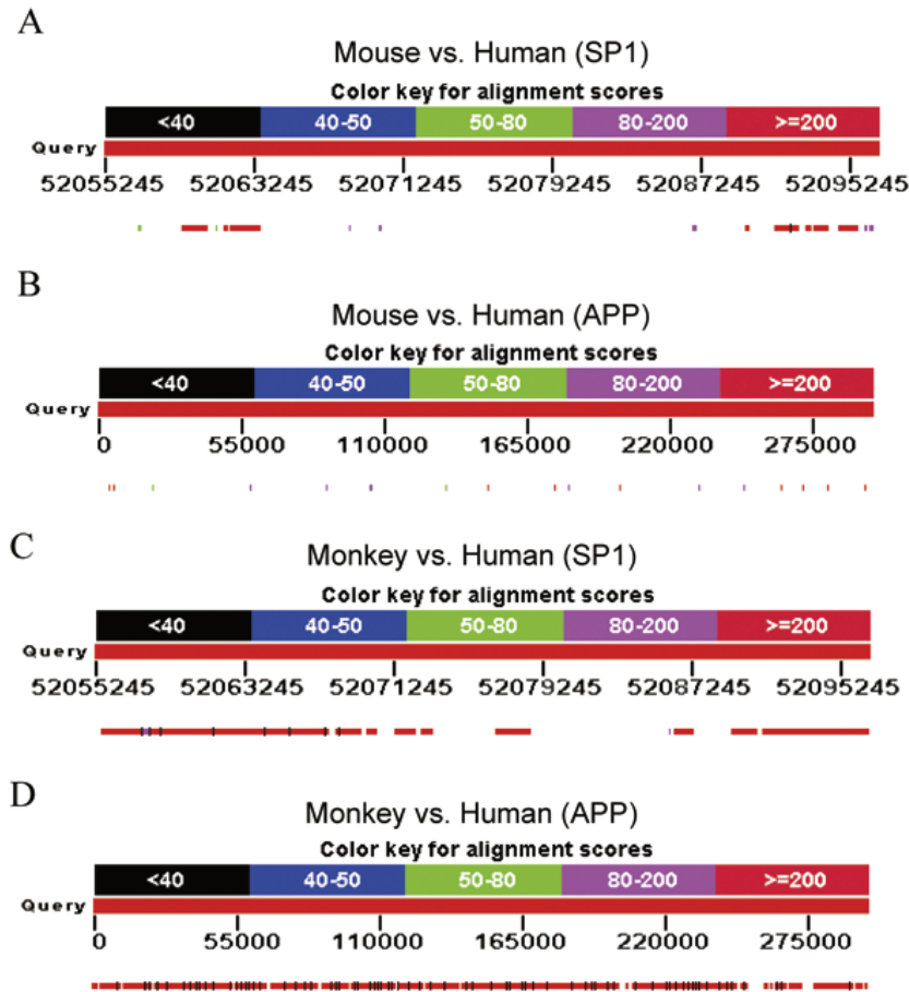
Fig. 6. Genomic homology of mouse SP1 and A \beta PP with human SP1 and A \beta PP. Genomic reference sequences for human SP1 and A \beta PP were used to BLAST the mouse reference genomic assembly as described in the text. Diagram represents coverage of homological regions over entire genomic sequences. Colors indicate percent homology as indicated by keys on figure. A) Homology of mouse SP1 versus human SP1. Numbers along alignment indicate position in human chromosomal genomic sequence [81]. B) Homology of mouse A \beta PP versus human A \beta PP. Numbers along alignment indicate position in human reference gene sequence [81]. C) Homology of monkey SP1 versus human SP1. Numbers along alignment indicate position in human chromosomal genomic sequence [81]. D) Homology of monkey A \beta PP versus human A \beta PP. Numbers along alignment indicate position in human reference gene sequence [81].
