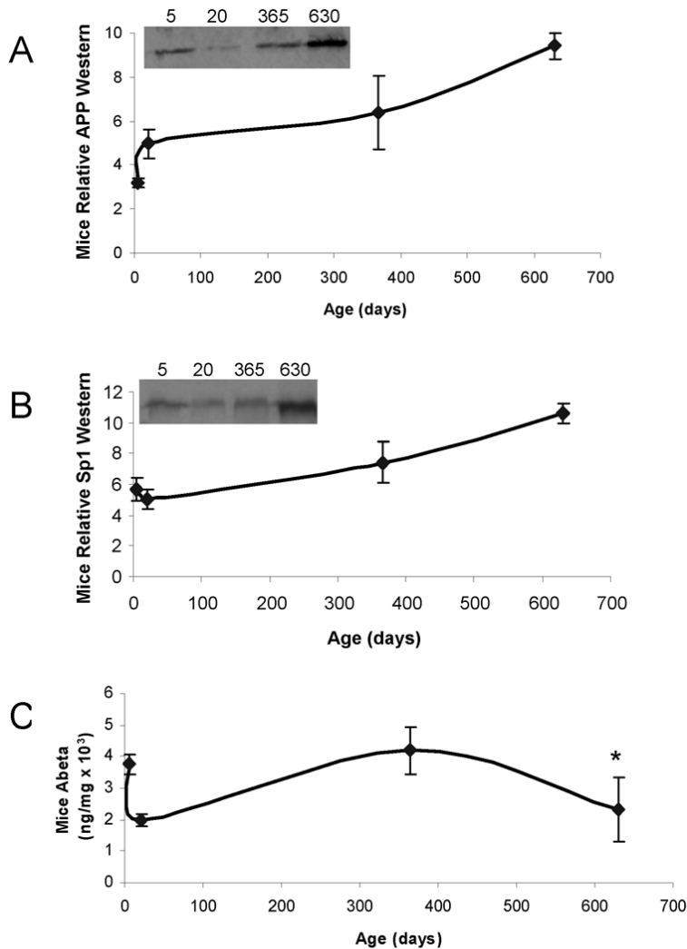
Fig. 2. Lifetime profile of AD related proteins ( A\beta PP, SP1, A\beta ) in the mouse brain. Protein from cortical tissue of wild-type mice was isolated, equal protein amounts were loaded and probed with 22C11 A\beta PP N-terminus antibody with SDS-PAGE western blot analysis as described in the methods section. The SP1 antibody used is mentioned in the methods section. Protein was also used to measure A\beta_{1-40} by a sandwich ELISA assay (IBL, Japan). Four time points are shown. Representative blots are shown in insets for western analysis. A) Relative A\beta PP levels; B) Relative SP1 levels; C) A\beta_{40} levels. Each data point in the curve is the mean + SEM ( n = 3 animals). “*” denotes significant difference between A\beta levels at PND 630 as compared to PND 365. Western blot results were normalized to \beta -actin signal.
