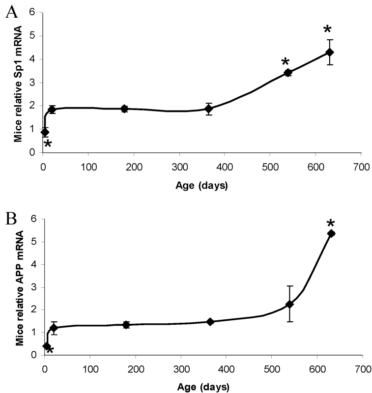
Fig. 1. Lifetime mRNA expression changes in AD related genes (SP1, A \beta PP) in the mouse brain cortex. Relative quantification was measured by using 7500 Real-Time PCR System (Applied Biosystems, CA) with \beta -actin serving as the endogenous control. A) Relative SP1 mRNA signal. B) Relative A \beta PP mRNA signal. Each data point in the curve is the mean + SEM ( n = 3-4 animals). “*” denotes significant difference for SP1 or A \beta PP mRNA time point when compared to that of PND 365.
