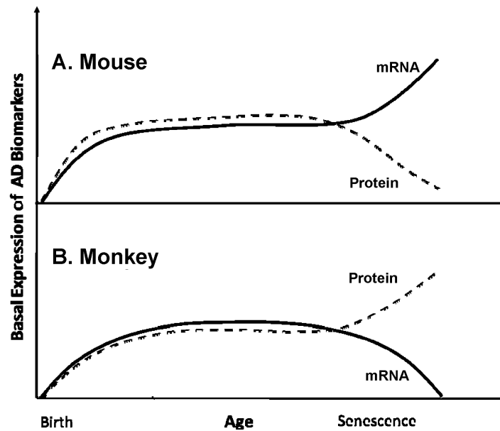
Fig. 8. Relationship between mRNA and protein product levels of selected AD-related genes in mouse versus monkey. Diagram illustrates levels of mRNA versus protein product levels of SP1 and A \beta PP in animal models studied. Solid line indicates mRNA levels over lifespan while dashed line indicates protein levels over lifespan. For each species, mRNA and protein levels diverge from each other in later life, albeit in opposite directions when comparing species to species. A) Mouse mRNA and protein levels. B) Monkey mRNA and protein levels.
