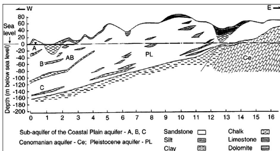
Fig. 2. Typical geological cross-section in the Gaza Strip [9].
