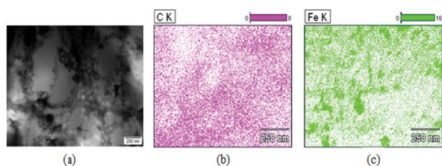
Fig. 2 (a) STEM micrograph, and elemental EDX mapping images (K lines) of the surface of chitosan fiber-supported nZVI particles (b) C, and (c) Fe.
