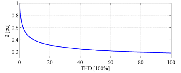
Fig. 5. The duty cycle versus THD.
