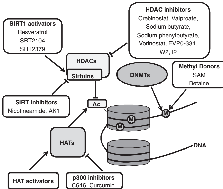
Fig. 1. Epigenetic targets and therapeutic approaches for AD. DNA methylation and histone modification mediators involved in AD and potential therapeutic interventions under development reported in literature. Barrels = histones; (M) = methyl group; (Ac) = acetyl group. Abbreviations in the figure are as follows: DNMT, DNA methyltransferase; HAT, histone acetyltransferase; HDAC, histone deacetylase; SIRT, sirtuin.
