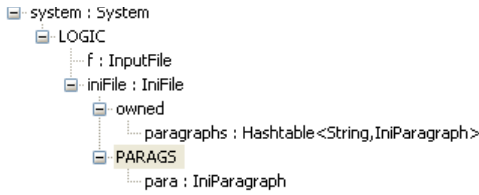
(a) Ownership tree, from the root object.
