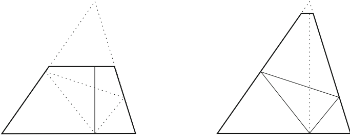
Fig. 7. Two possibilities for the orbits attaining \ell(T)
