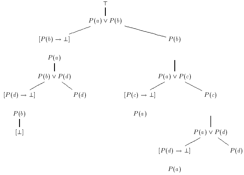
Figure 2: The Model Tree with Complement Splitting for Example 2.
