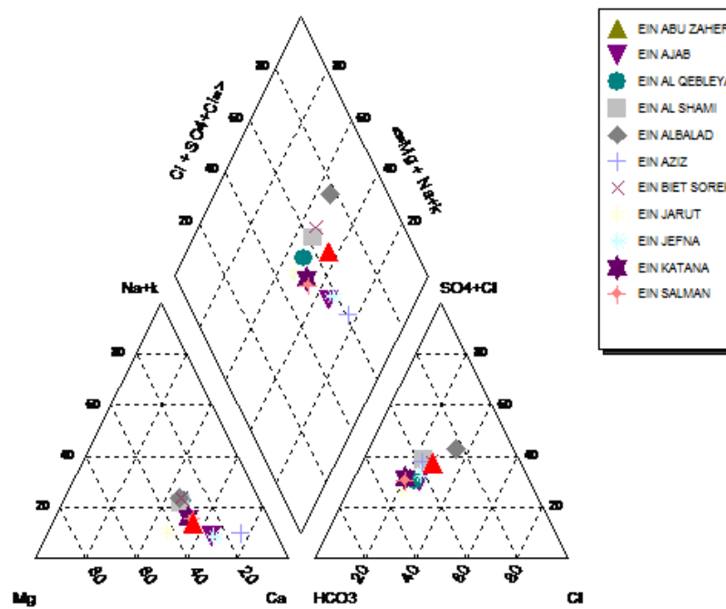
Fig.15: The Piper diagram in the wet period
